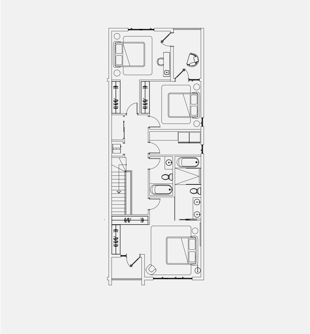
SECOND FLOOR: FROM 1,046 SQ. FT.
